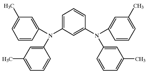
PDA
