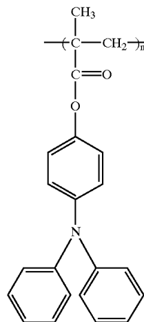
TPA-PMMA
