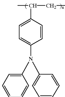
DPA-PS
