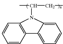
PVCz
