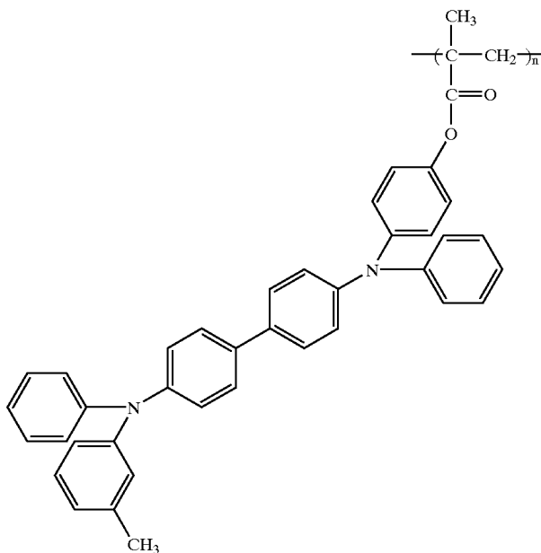
TPD-PMMA
