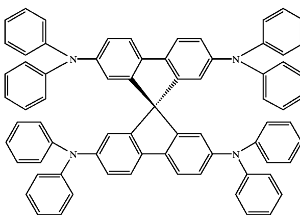
spiro-TPD
