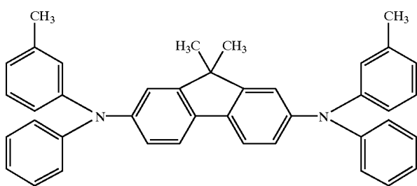
DTDPFL
